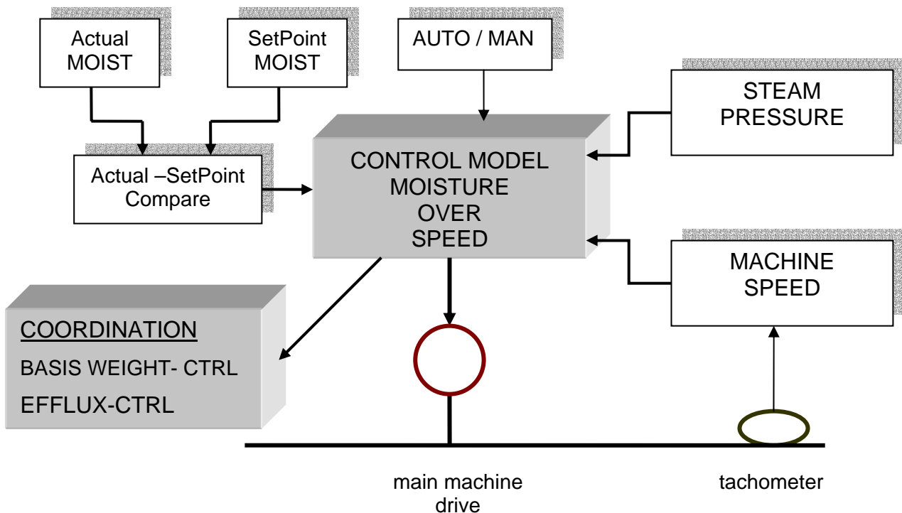
Moisture control over machine speed
